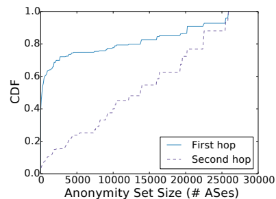
Figure 12: Anonymity Set Size
